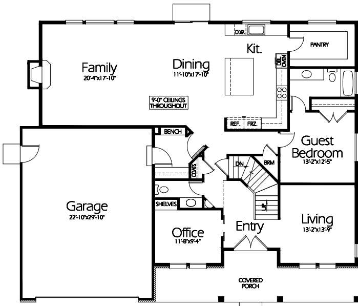
Main Level 1927 Sq. Feet
