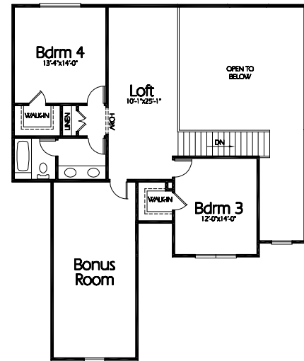
Upper Level 840 Sq. Feet
