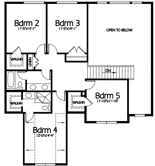
Upper Level 1104 Sq. Feet
