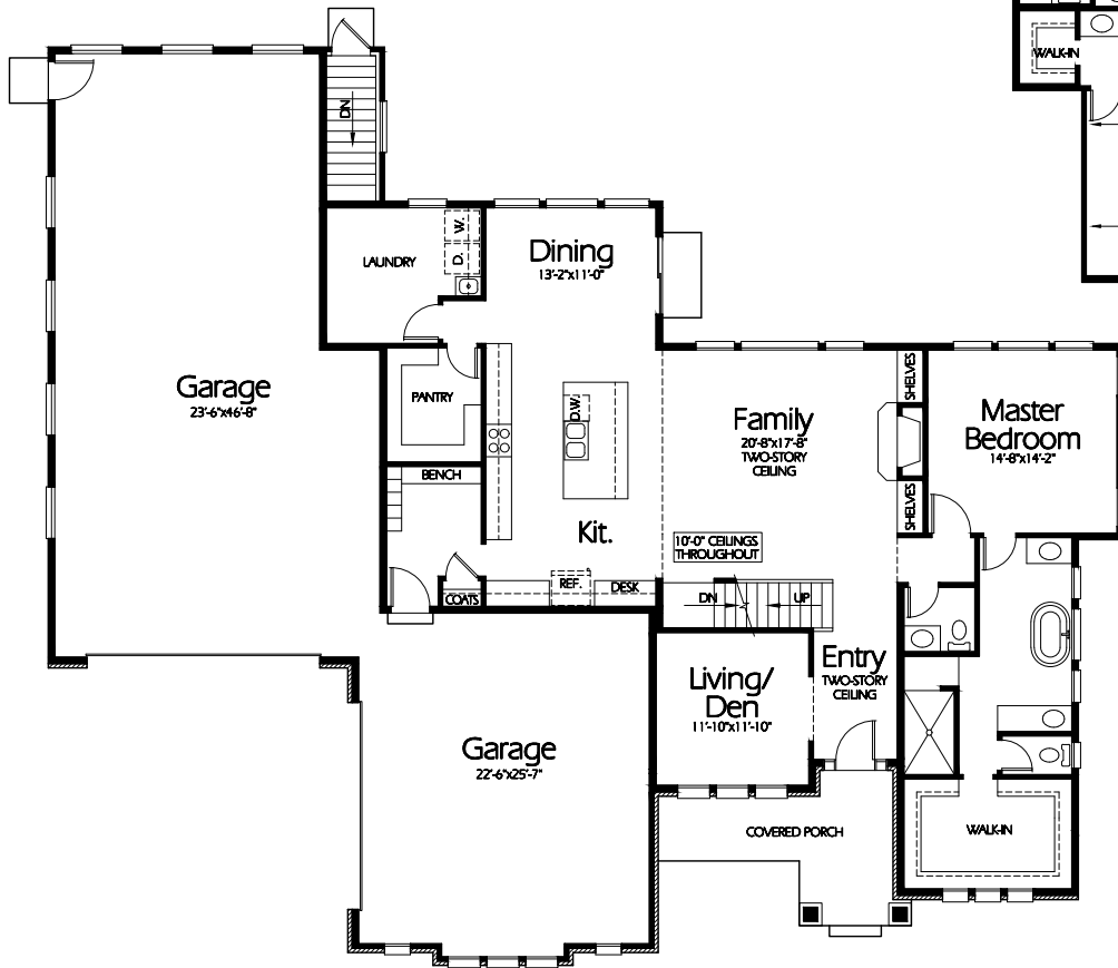
Main Level 2045 Sq. Feet
