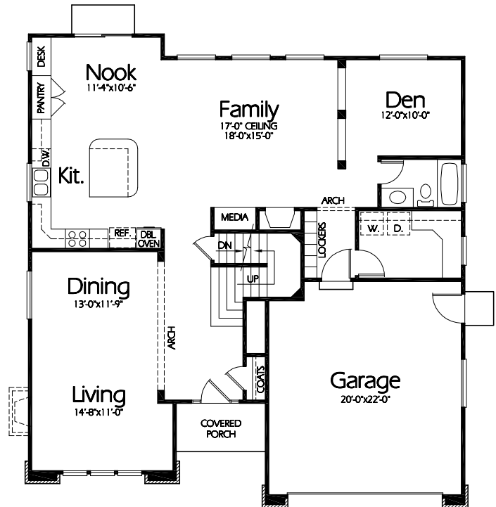
Main Level
