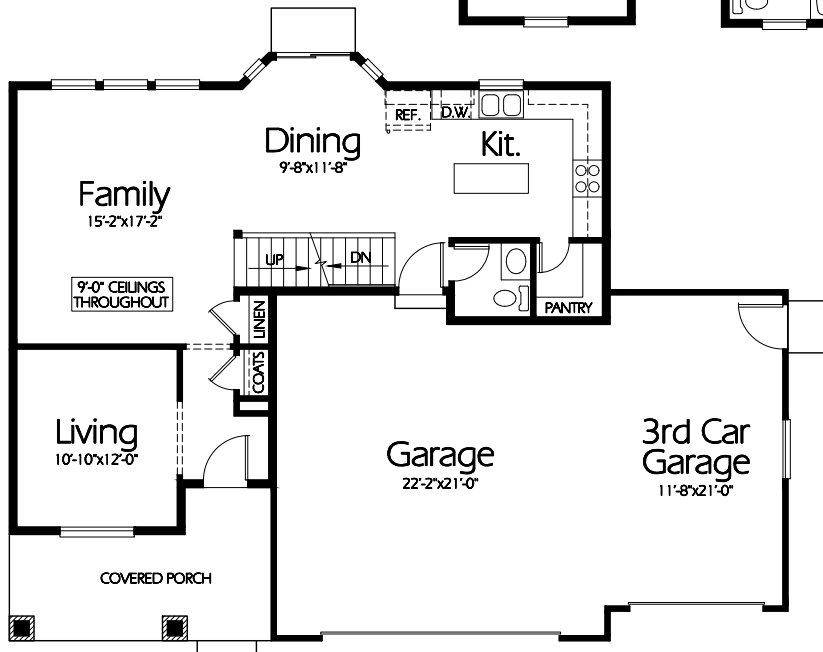
Main Level
