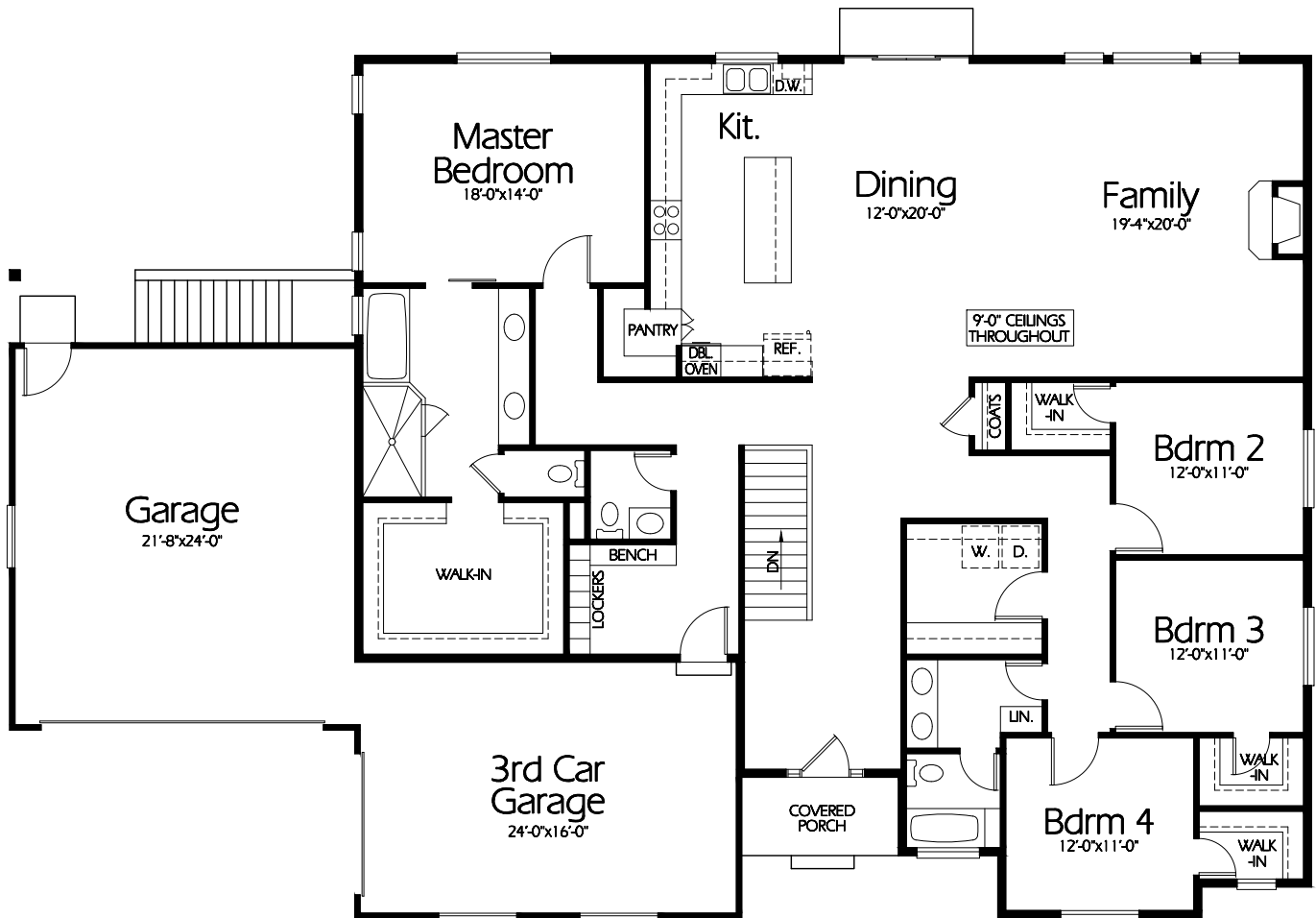
Main Level
