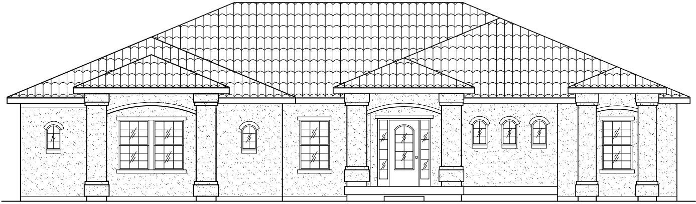
Front Elevation
