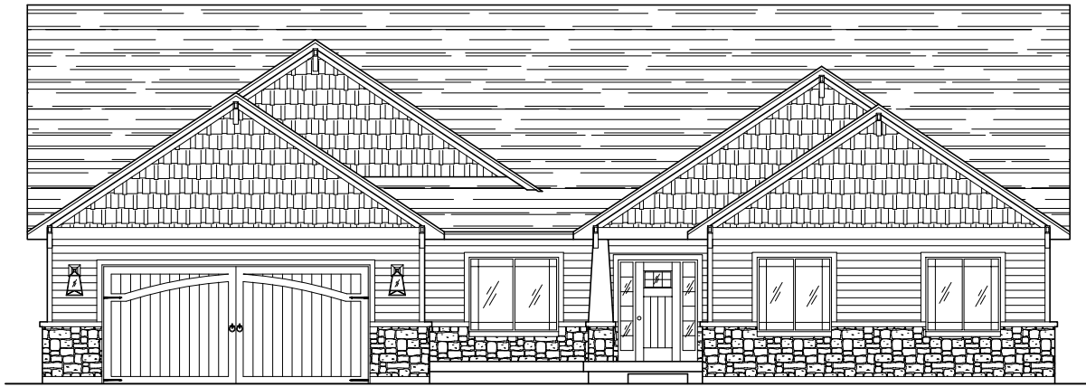
Front Elevation
