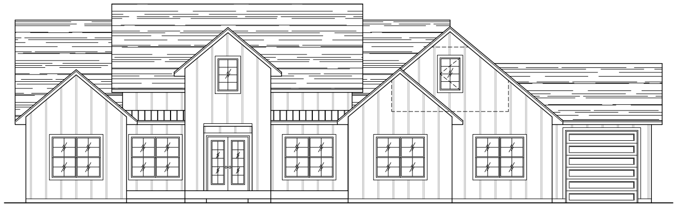
Front Elevation
