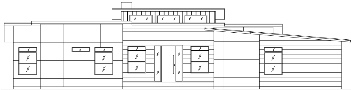
Front Elevation
