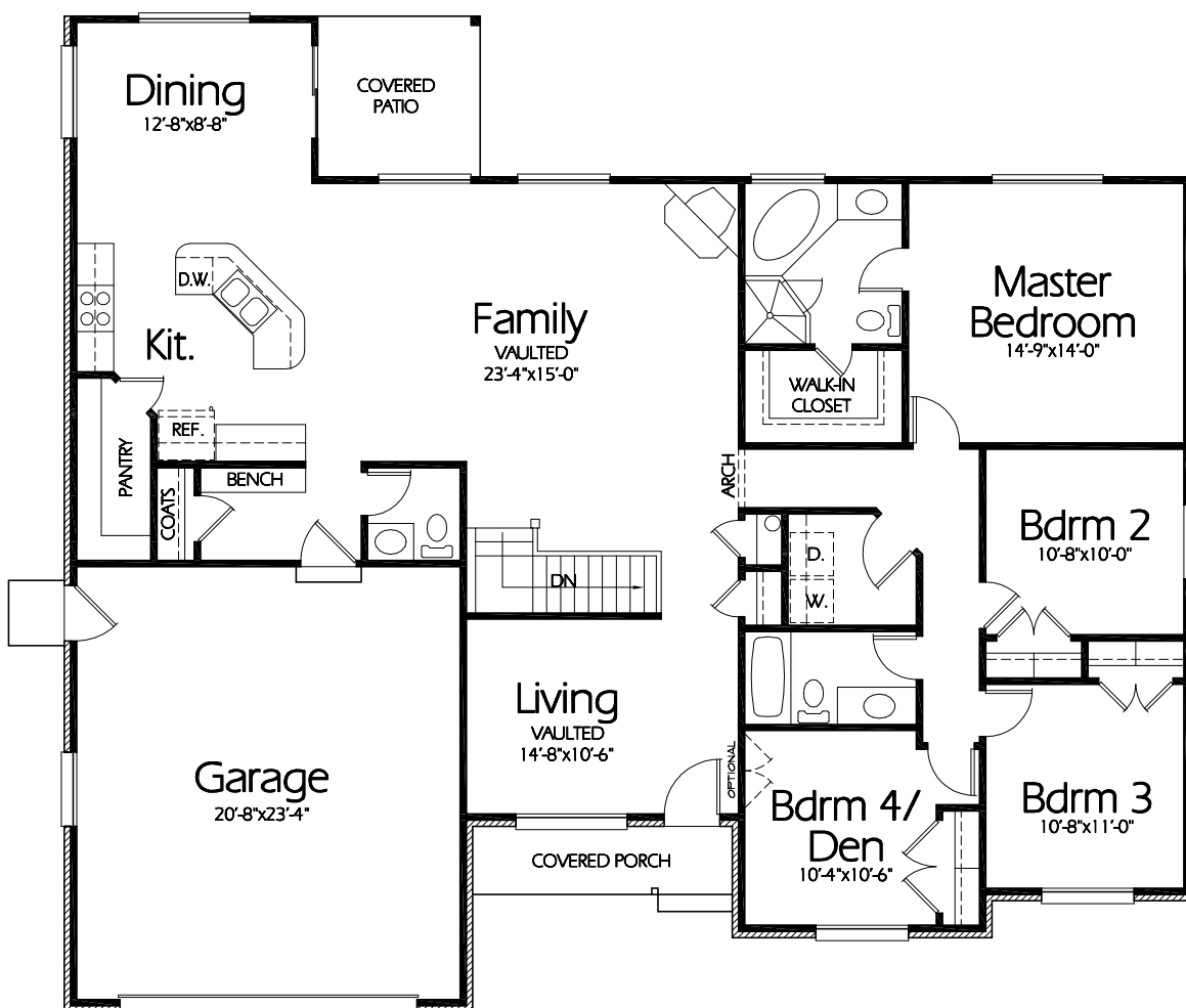
Main Level
