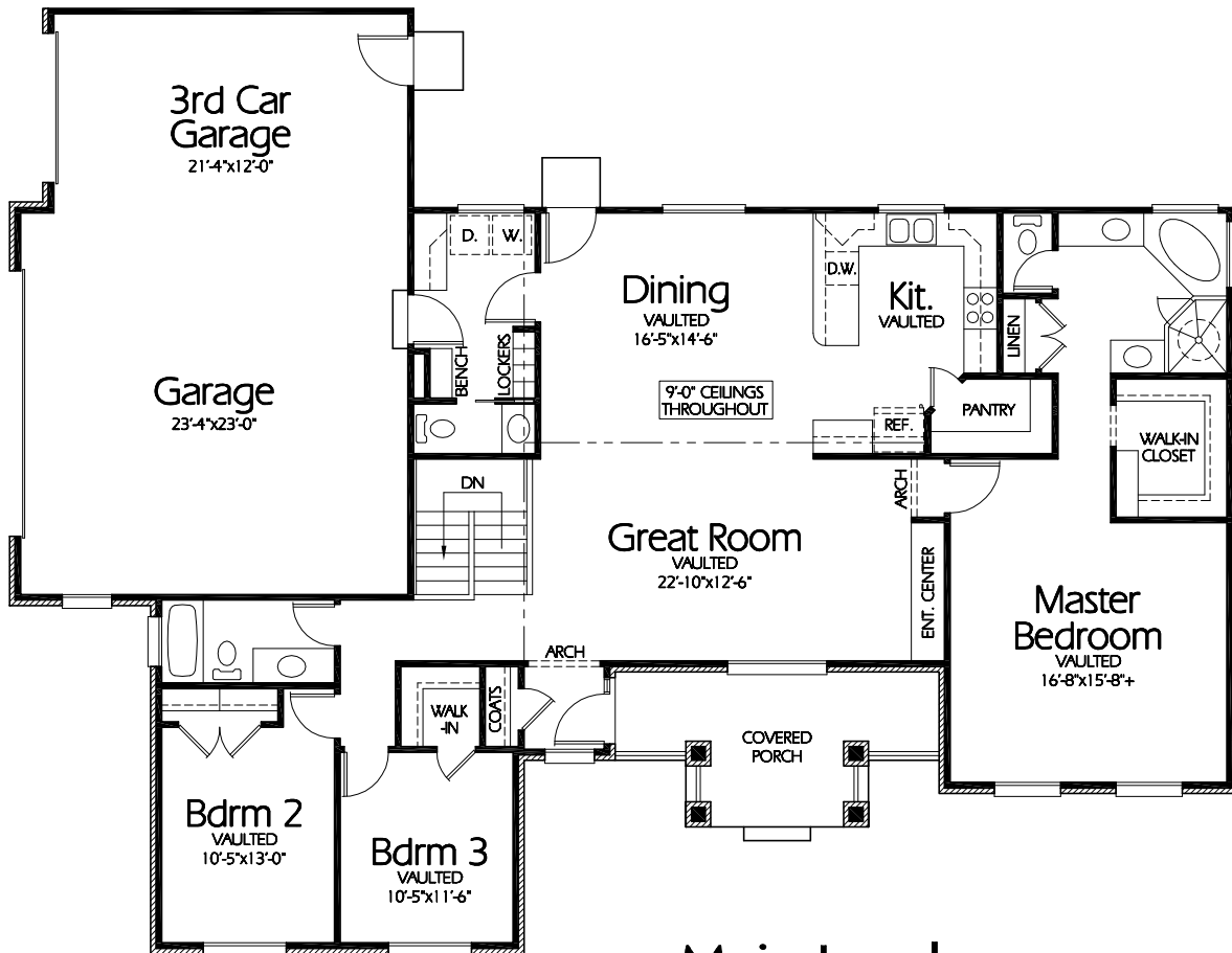
Main Level
