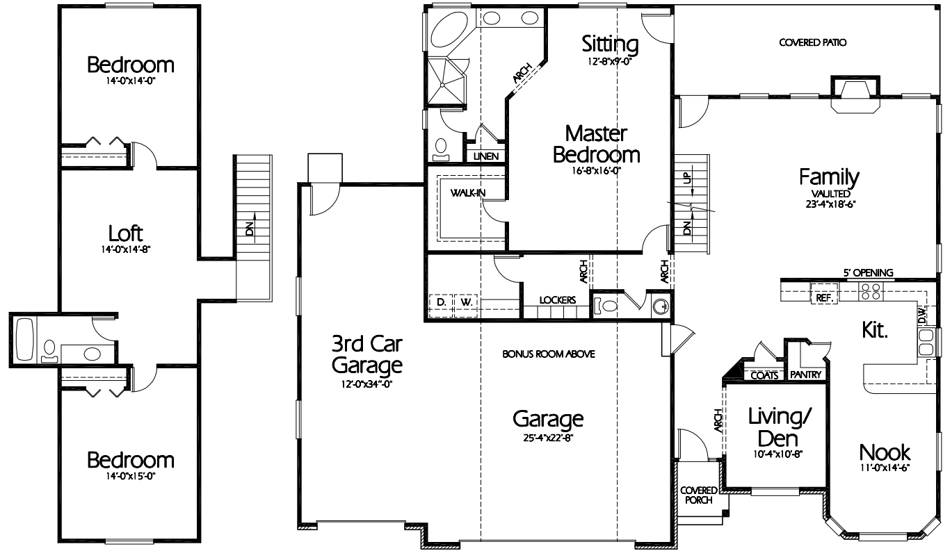
Upper Level (Bonus) 840 Sq. Feet
