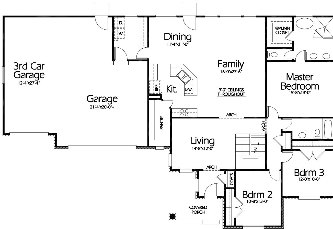
Main Level
