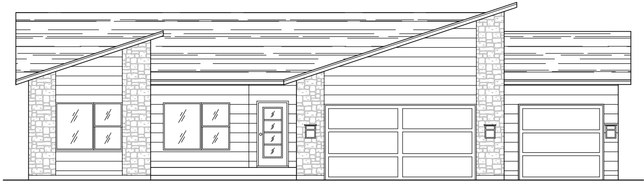
Front Elevation
