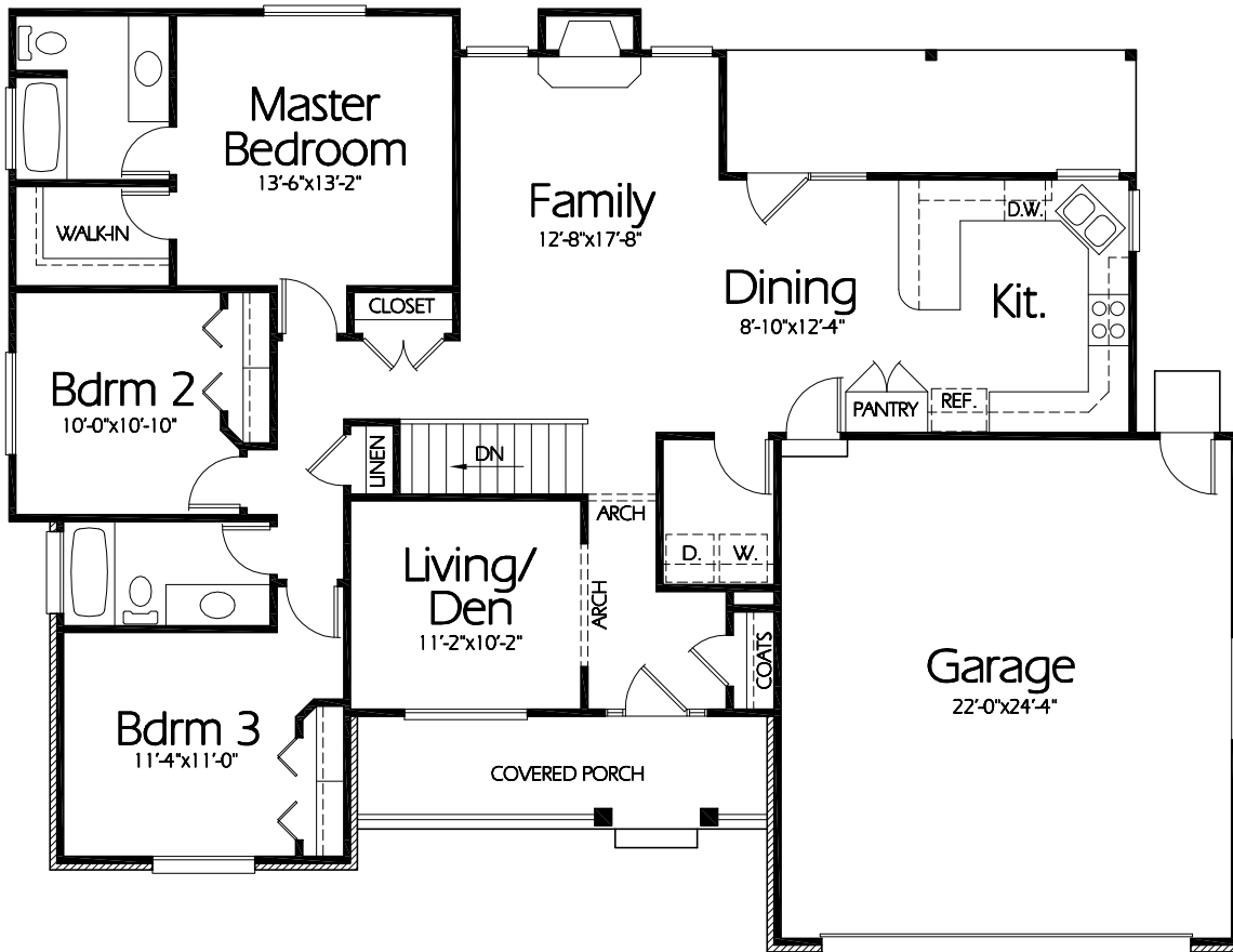
Main Level
