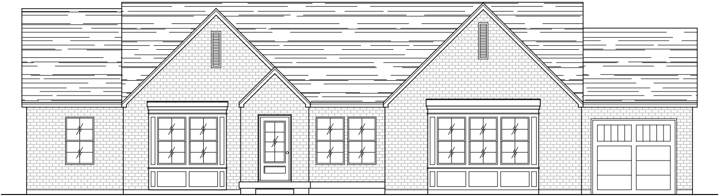
Front Elevation
