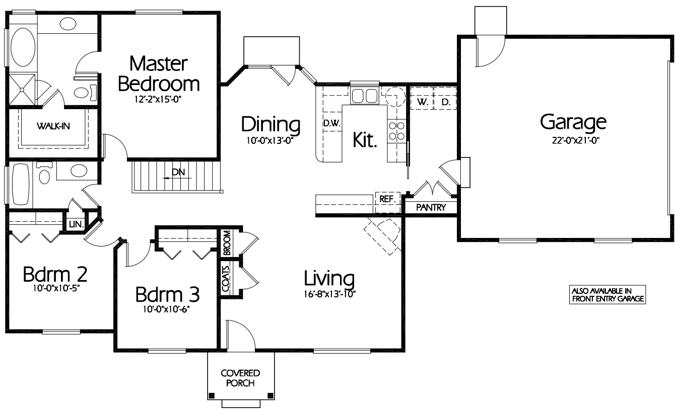
Main Level
