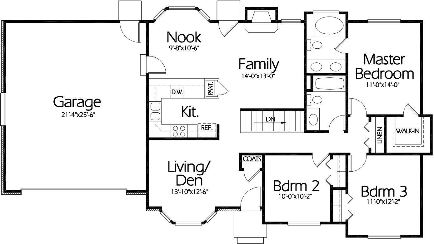
Main Level
