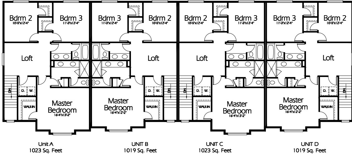
Upper Level 4092 Sq. Feet
