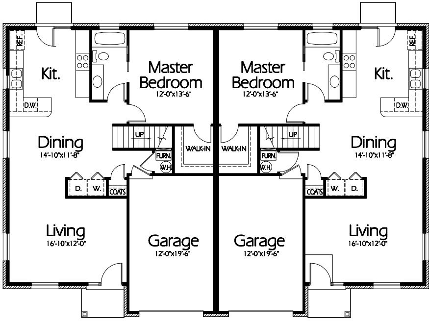
Main Level 1914 Sq. Feet
