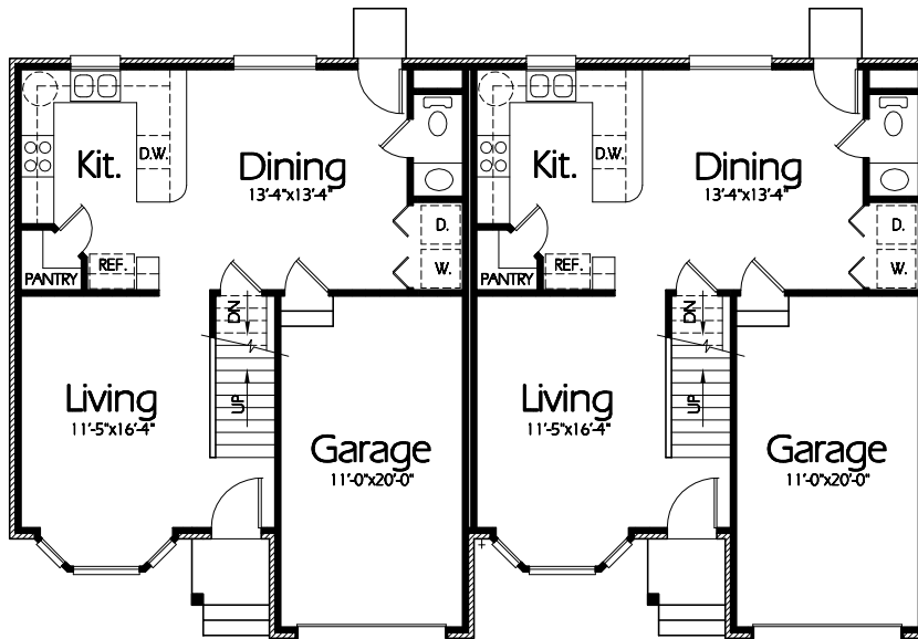
Main Level 1302 Sq. Feet
