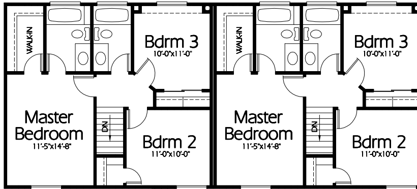
Upper Level 1336 Sq. Feet
