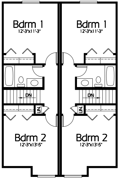
Upper Level 996 Sq. Feet 498 Sq. Feet per Unit
