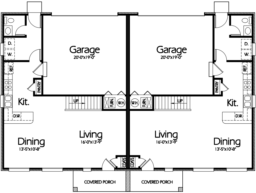
Main Level 1514 Sq. Feet 757 Sq. Feet per Unit
