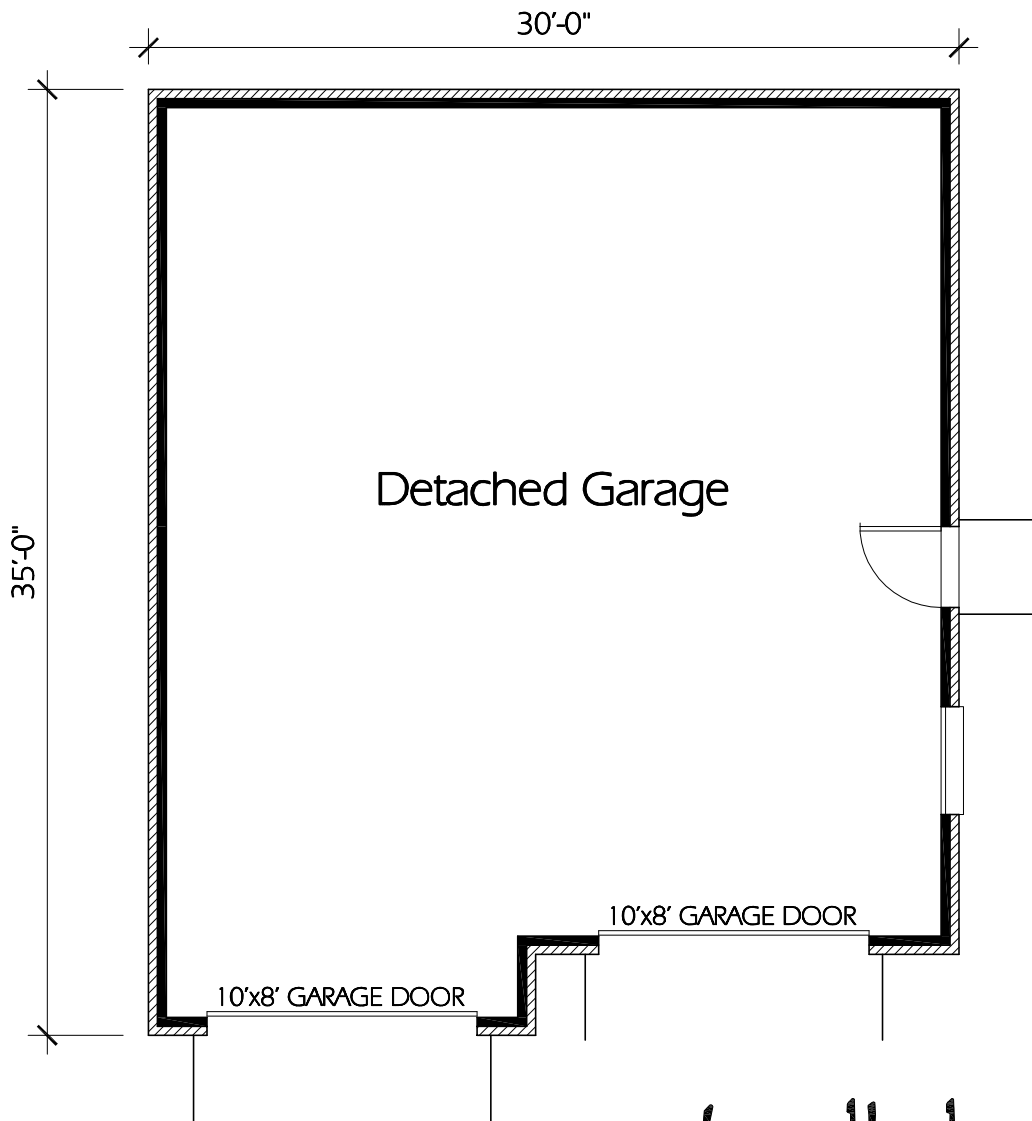
Garage 30'x35' Version A
