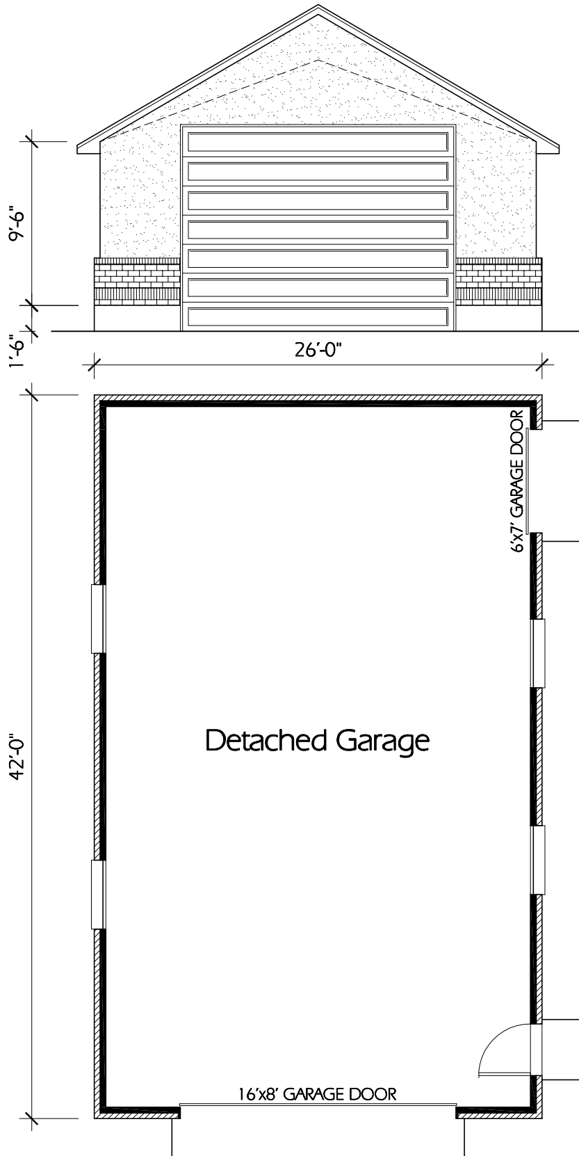
Garage 26'x42' Version A
