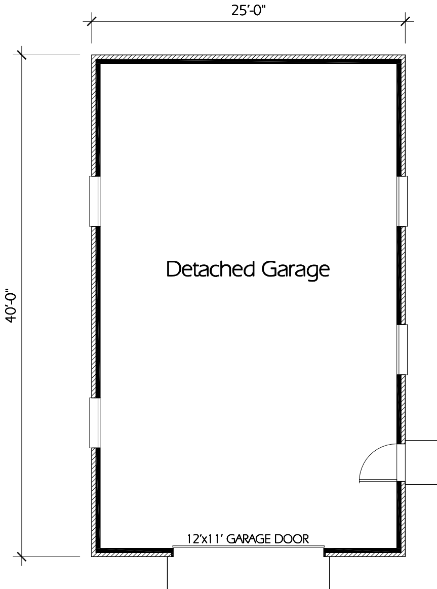
Garage 25'x40' Version A
