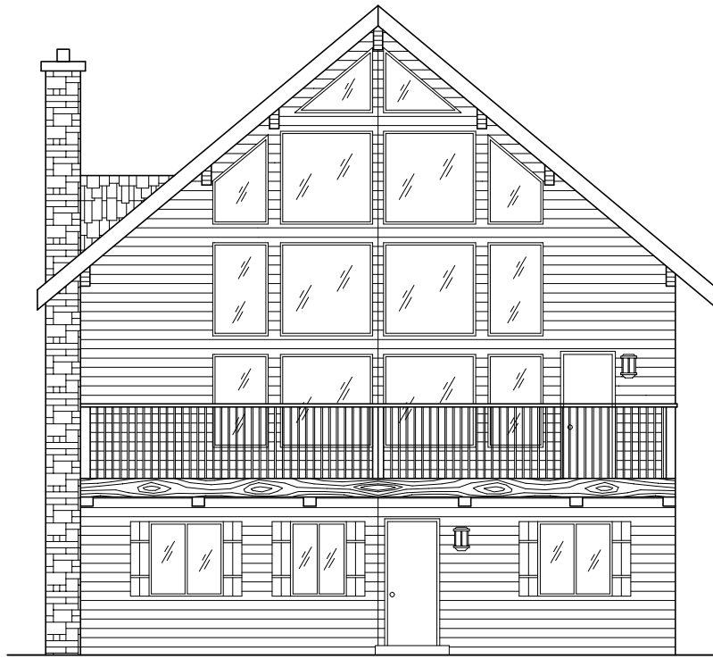
Front Elevation
